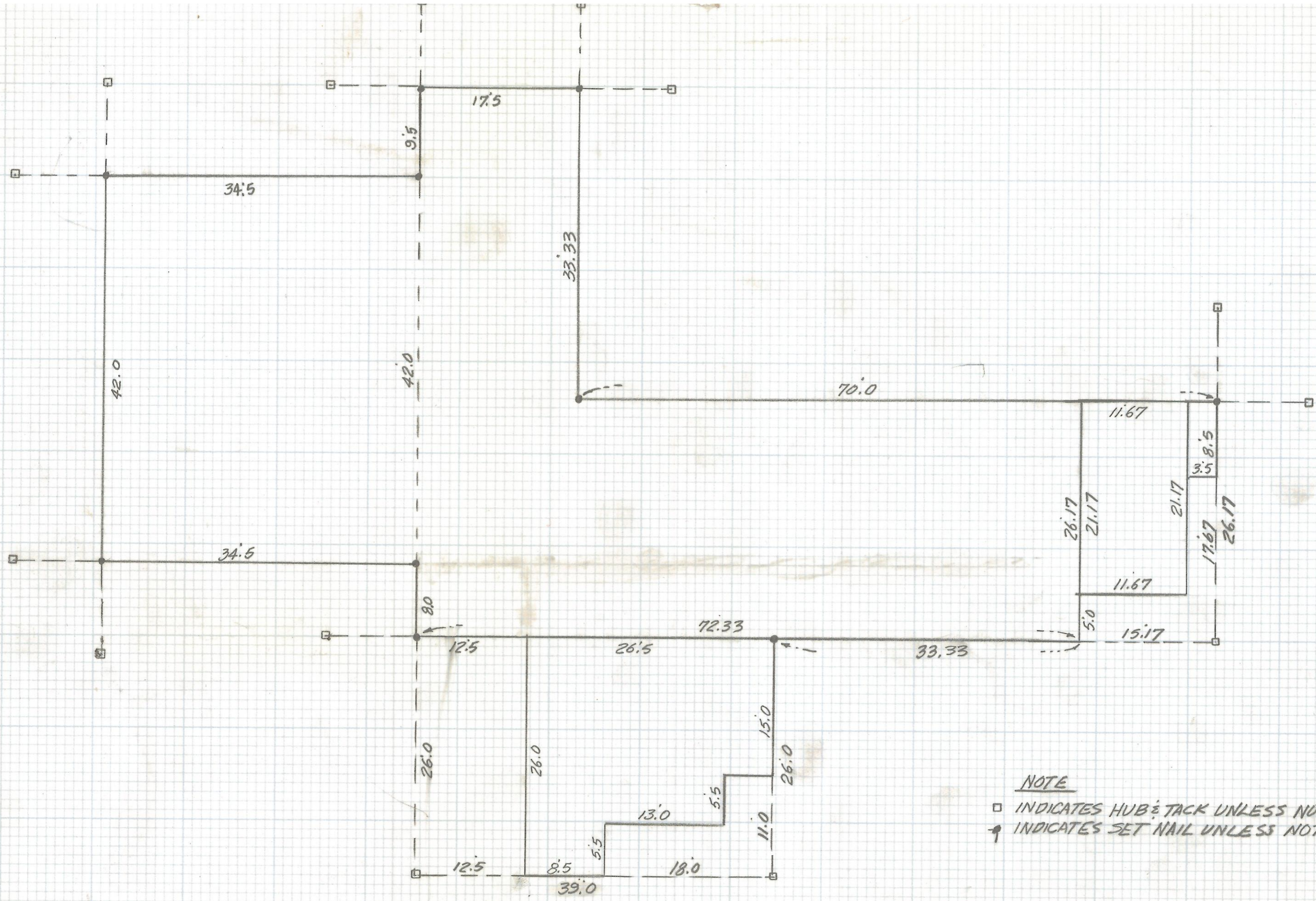
SKETCH OF ASCHER RESIDENCE FOR CONCRETE ON LOT 232 FINISTERRA BOOK 34 PAGE 26 MAPS & PLATS
