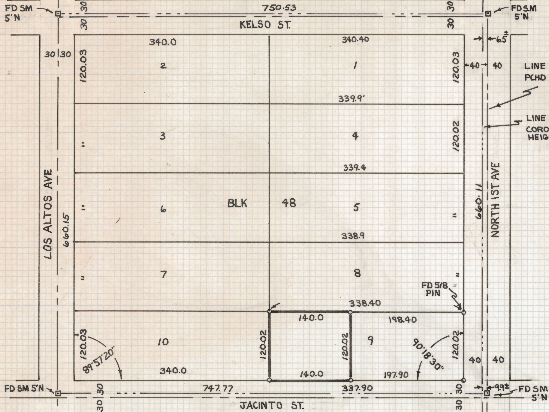
SCALE 1"=100' DETAIL OF LOT 9
