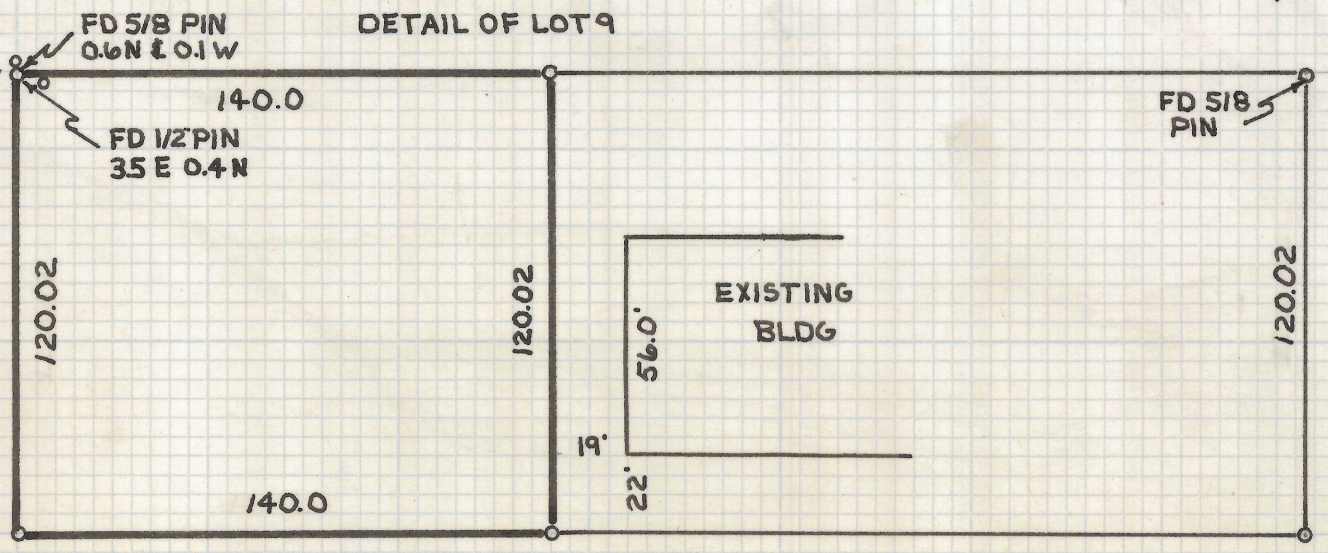
SCALE 1"=50'
